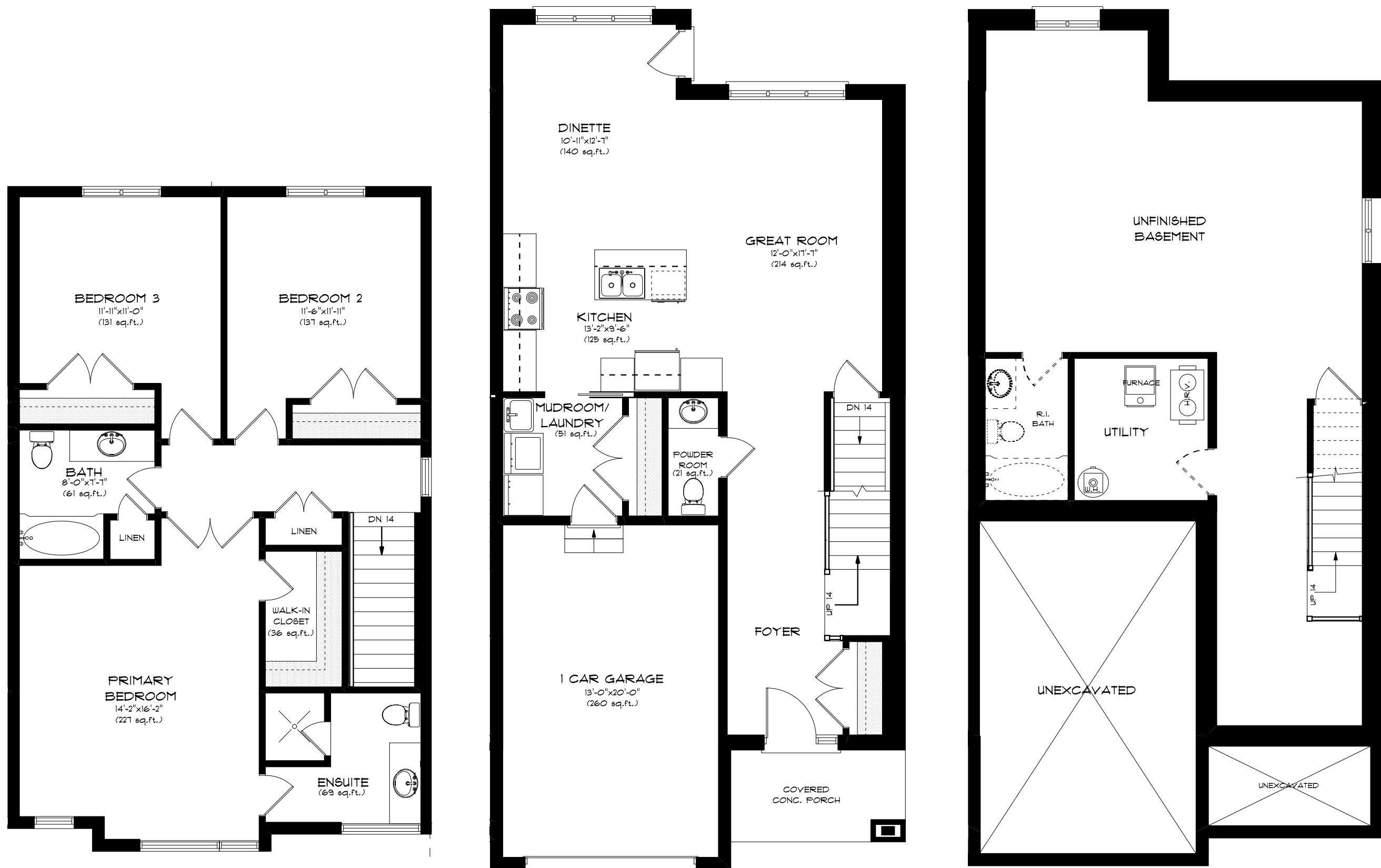
▲ SECOND FLOOR
