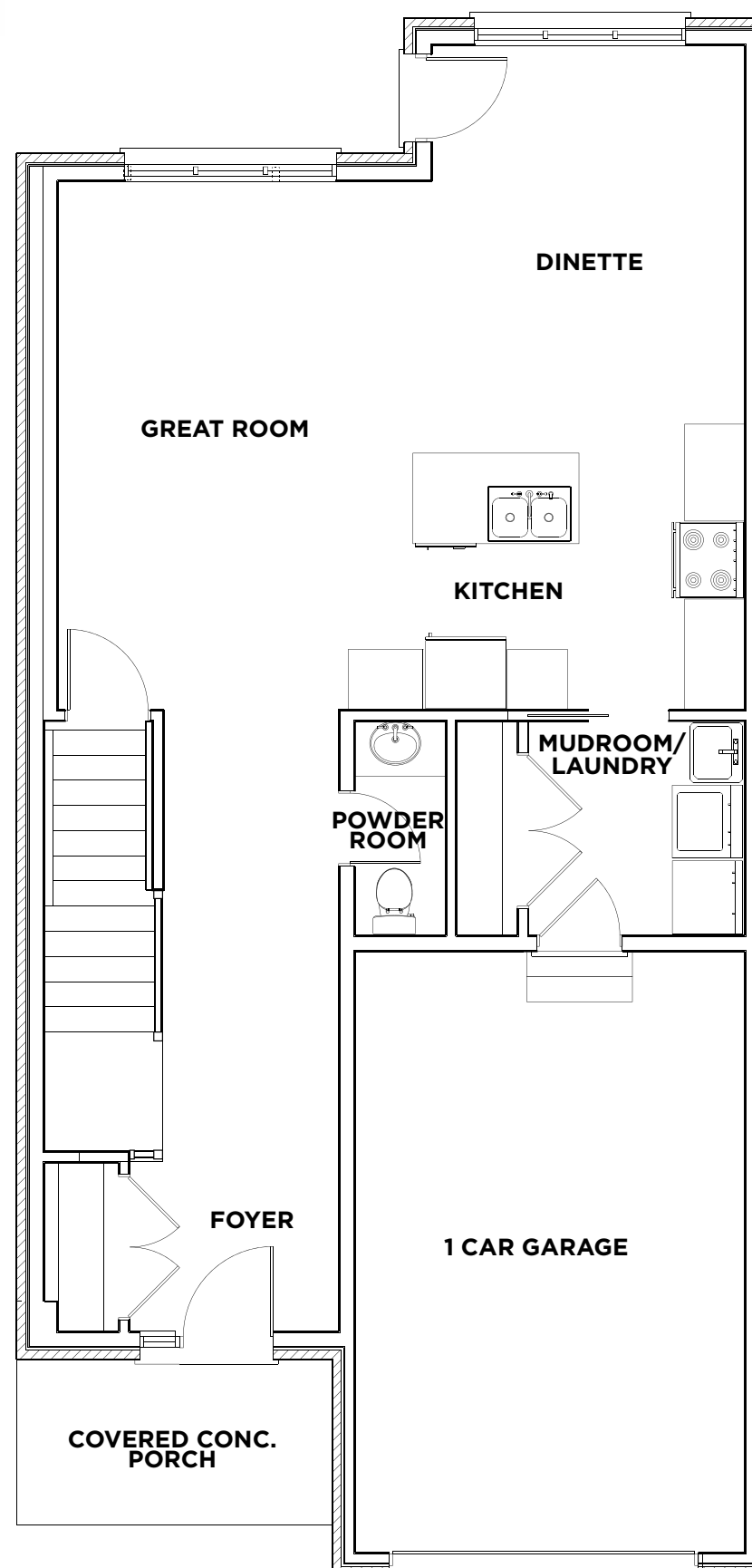
▲ MAIN FLOOR
