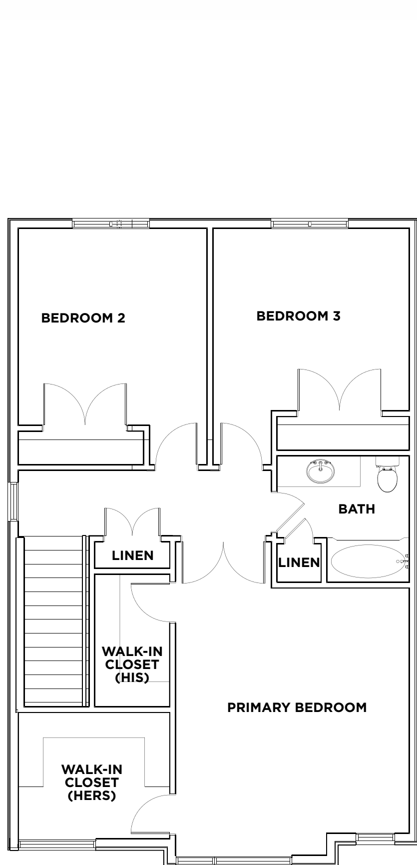
▲ SECOND FLOOR
