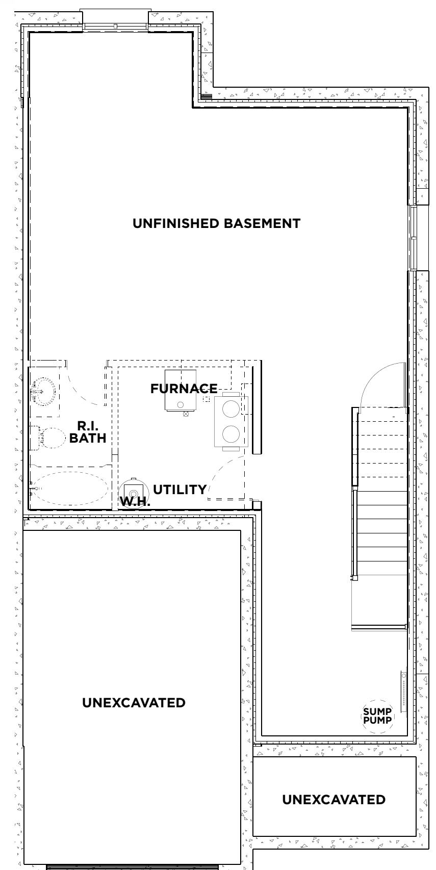
▲ BASEMENT
