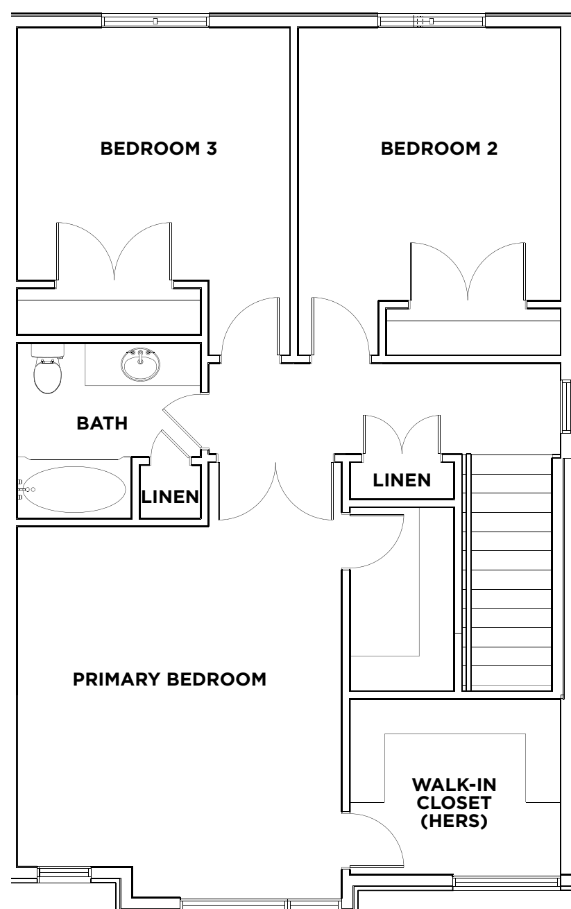
▲ SECOND FLOOR
