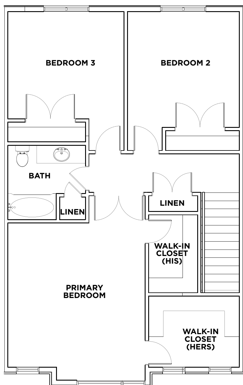
▲ SECOND FLOOR
