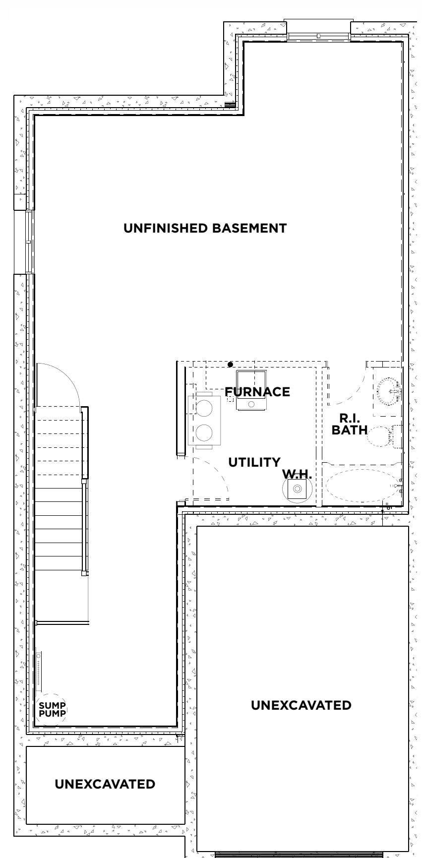
▲ BASEMENT
