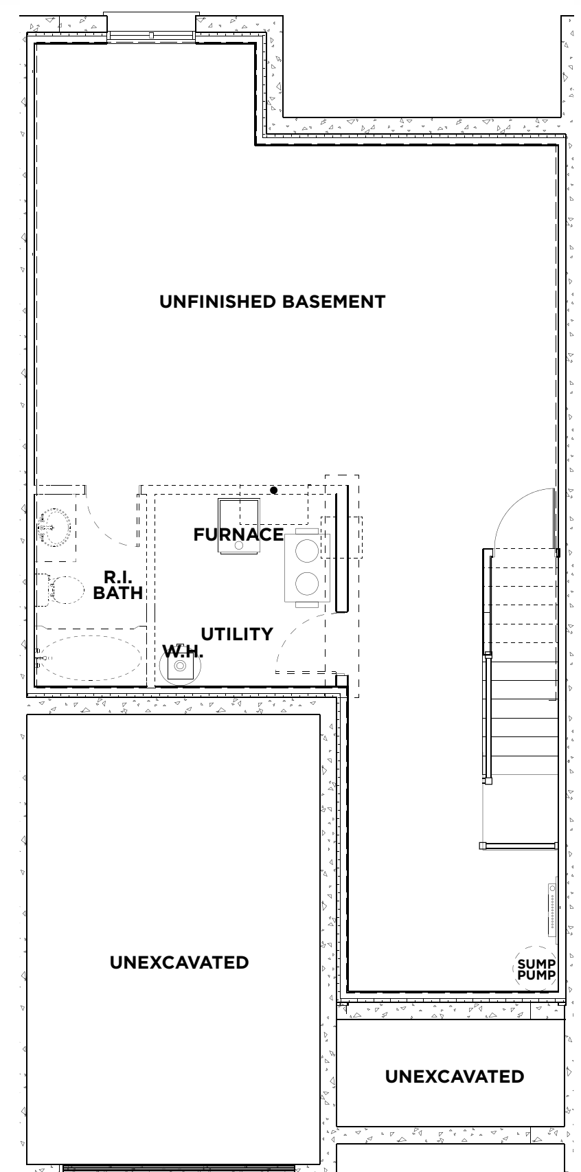
▲ BASEMENT
